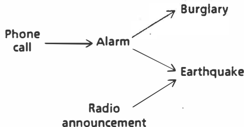
Figure 2: An inference network for Mr. Holmes' situation
